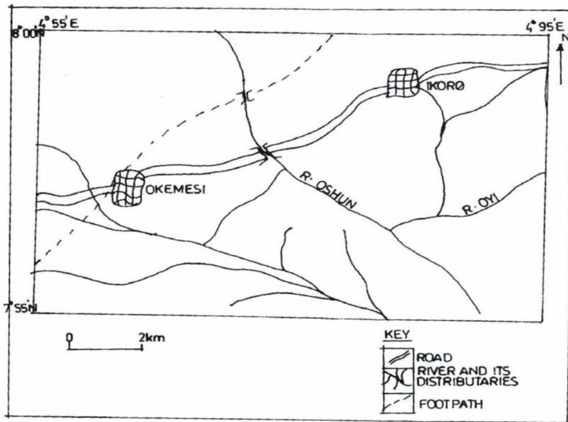
Fig.2. Trellis drainage pattern of the study area.
